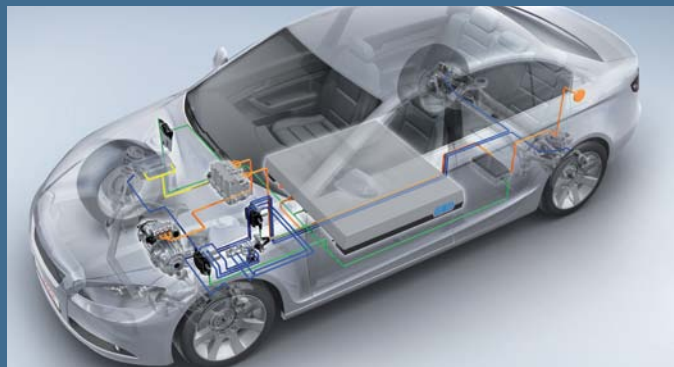
Electric vehicle with vacuum-independent regenerative braking system
