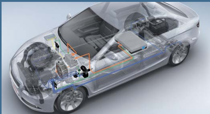
Hybrid vehicle with vacuum-based regenerative braking system
